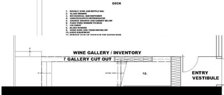
MAIN FLOOR PLAN - WALK THROUGH GALLERY
