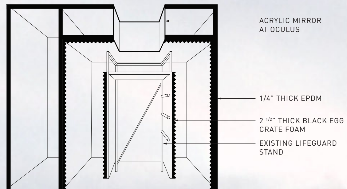
SECTION 1:50
